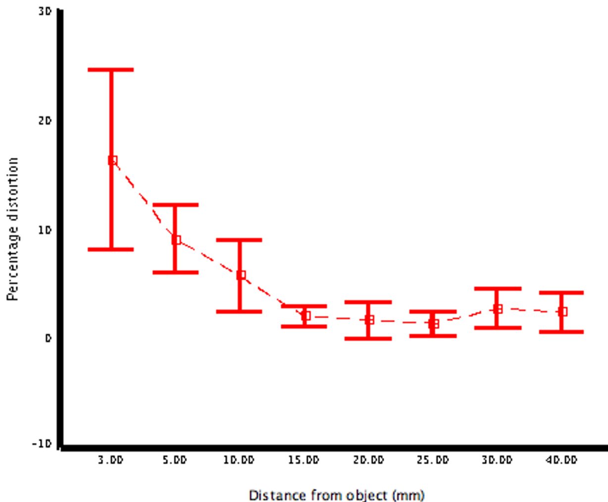
Figure 6 Mean central distortion ± 95% CI for the central or geometrical axis aligned bronchoscope.
